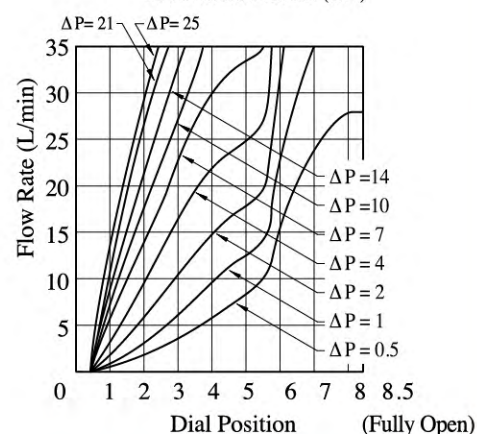
開度-流量特性 Metred Flow vs. Dial Position ΔP : Differential Pressure (MPa)
