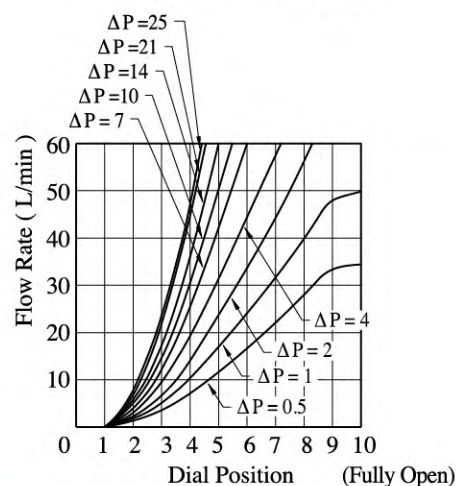
開度-流量特性 Metred Flow vs. Dial Position ΔP : Differential Pressure (MPa)
