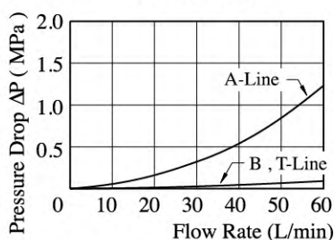
壓力降特性 Pressure Drop
