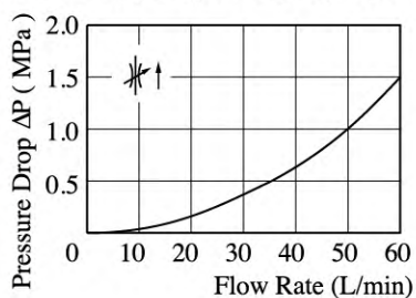
調整輪全開時壓力降特性 Pressure Drop at Spool Fully Open (P-Line)
