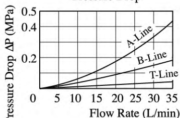
壓力降特性 Pressure Drop
