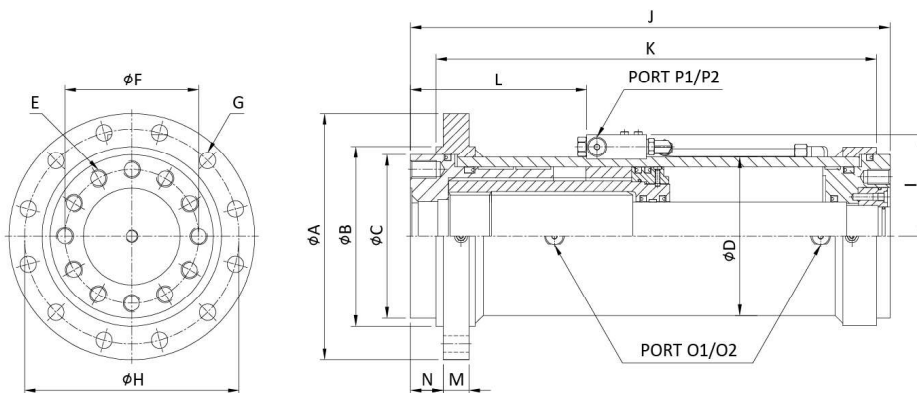
RA30-Rod and Mounting Flange
